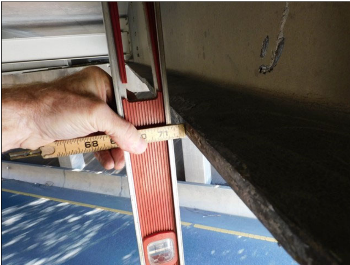
Span 2 Beam 9: ALONG BOTTOM FLANGE AT MID SPAN, AREA OF IMPACT DAMAGE [6 FOOT LONG] WITH DEFLECTION [UP TO 1/2 INCH].
